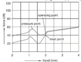
MX with tactile feel(ergonomic) (Brown)
