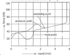
MX with click tactile feel (Blue)
