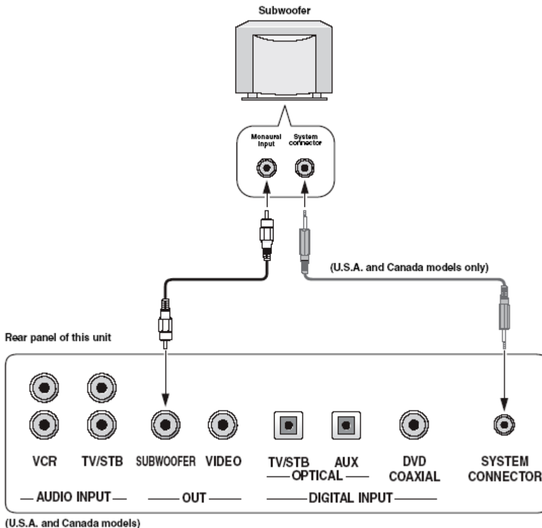
System connector cable (supplied with the YAMAHA subwoofer with the SYSTEM CONNECTOR jack)
