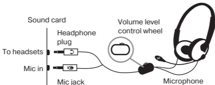
Fig. 1. Connection diagram
