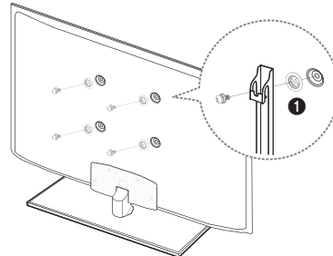
Case B. Installing another company's Wall-Mount
